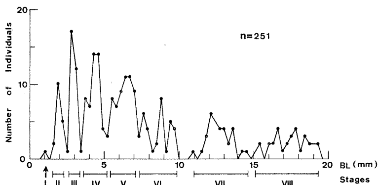
Fig. 3. Body length composition of Scyllarus kitanoviriosus larvae in the western Wakasa Bay from August to November, 1983.
